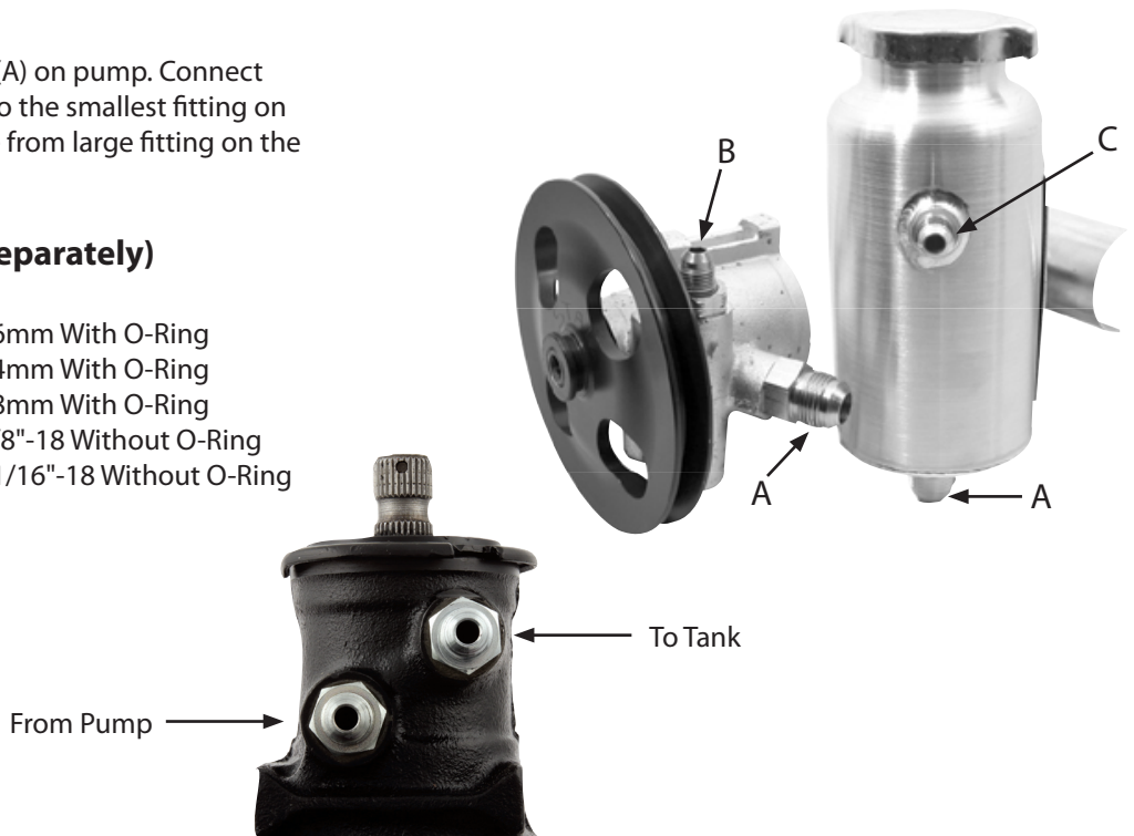
Typical GM 800 Series Steering Box Connection
