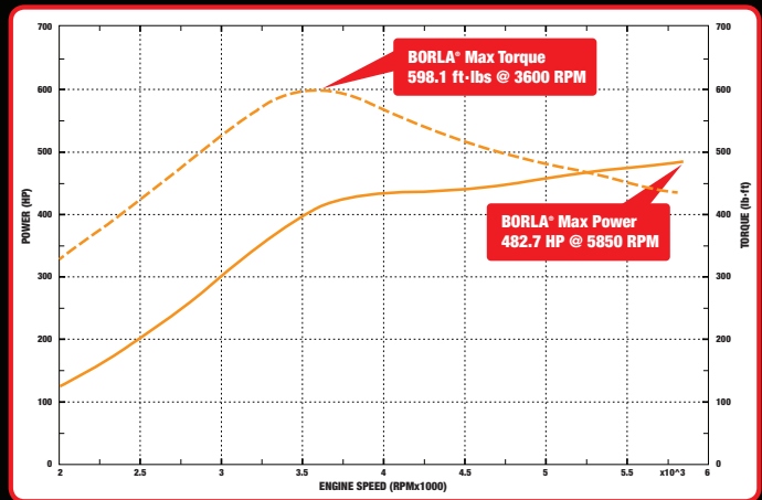
2016 Ford F150 3.5L DYNO RESULTS
